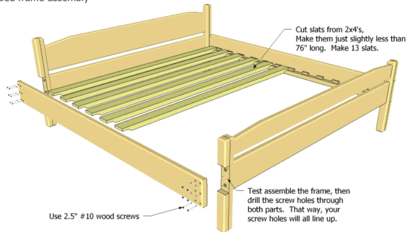
Bed frame assembly
